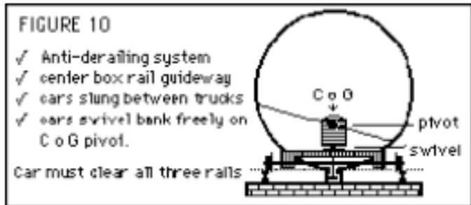
Center box rail, ability to “lean” minimize derailments
